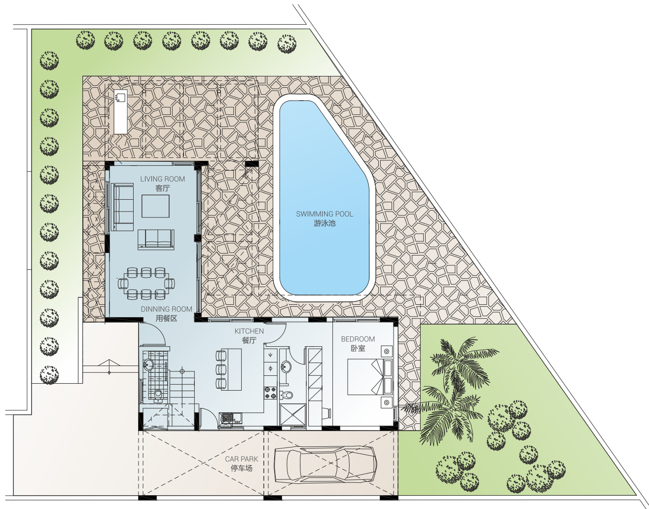
GROUND FLOOR | 地面层
